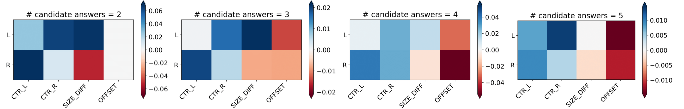
Figure 8: Feature weights learned by logistic regression for predicting click rate when two adjacent candidate answers are swapped. The figure should be viewed in color.
