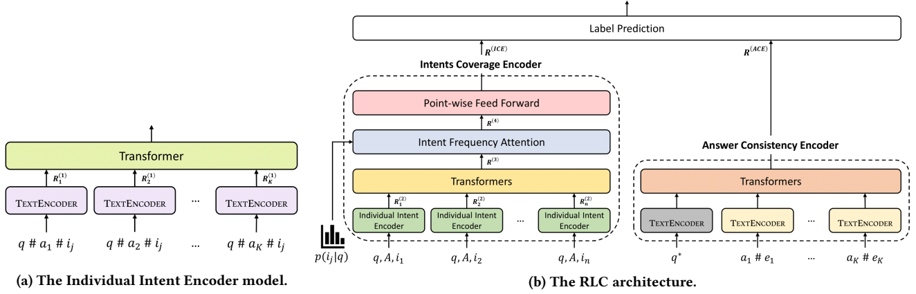
Figure 9: The neural network architecture for RLC. Same color indicates shared parameters.
