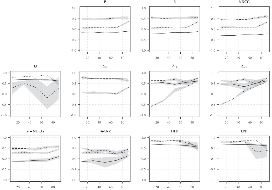
Fig. 3. Correlation with commonality when downsampling all categories. Horizontal axis (all plots): percent-age downsamped. Vertical axis (all plots): \tau correlation with commonality. Top row: Utility metrics; middle row: fairness metrics; bottom row: diversity metrics. Solid line: movies; dashed line: music; dotted line: literature. Lines show mean across five trials. Shaded regions indicate one standard deviation around the mean.
