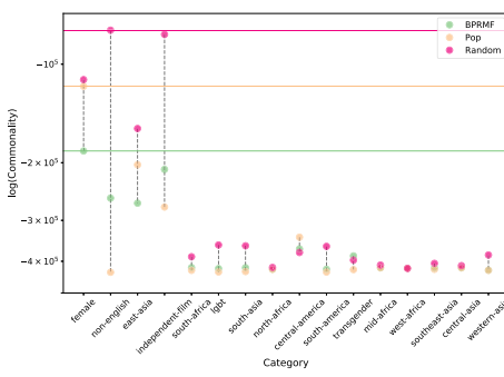
(a) Commonality for MovieLens-1m
