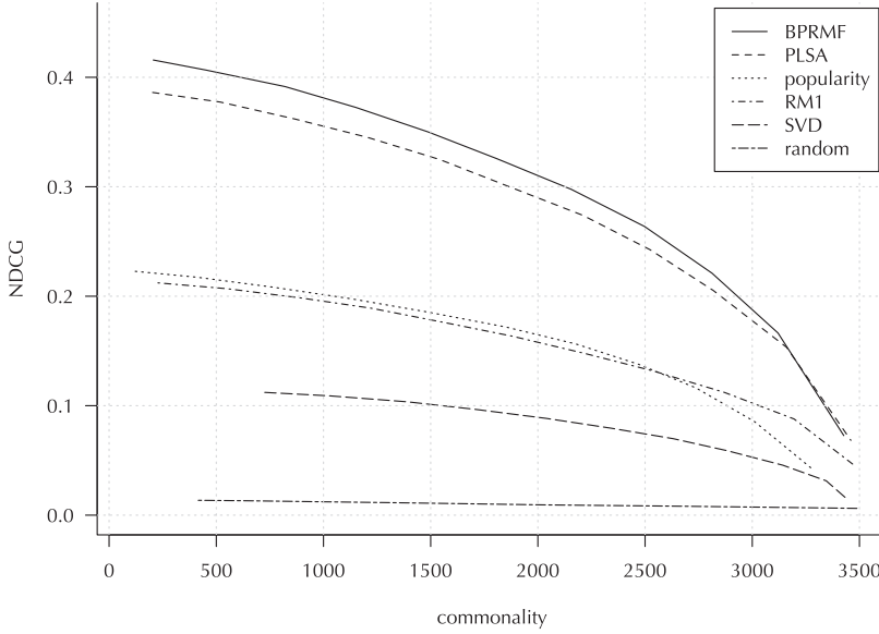
Fig. 6. Utility-commonality tradeoff using interleaved promotion. Commonality and NDCG of personalization-focused algorithms post-processed by interleaved promotion. Results for the movies domain.
