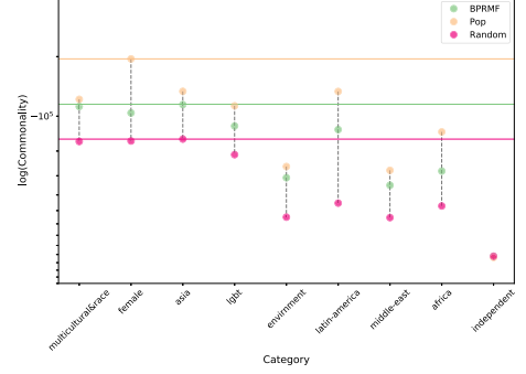
(b) Commonality for libraryThing
