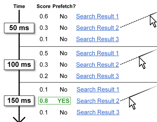
Figure 1: Example of cursor-based prefetching. The model estimate of whether the searcher will select one of the top three results over time (at 50ms, 100ms, 150ms) is shown alongside each link (as Score ). These estimates change as a function of the searcher's cursor movements. The cursor trail and the trajectory towards the second result are highlighted in the figure with solid and dashed lines respectively. When the model score for a result reaches a certain threshold (0.8 for Search Result 2), that result is prefetched.
