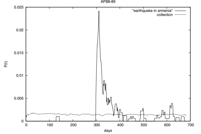
Figure 1: Temporal profile, P(t|Q) , of the query “earthquake in armenia” using the AP88-89 collection. The collection distribution, P(t|C) , is shown for reference.
